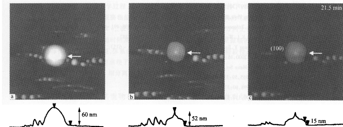
Fig. 3 in situ AFM images of tip-induced crystallization of PEO ( M_n = 1.0 \times 10^4\ \text{g/mol} ) on the mica surface by nanoindentation
