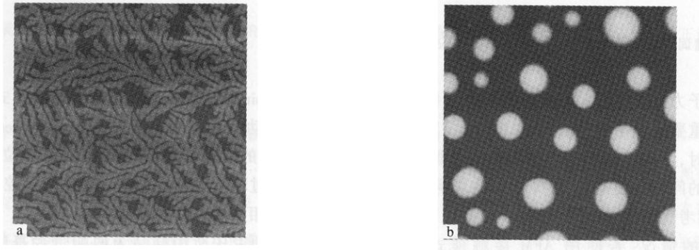
Fig. 1 Typical AFM height images of (a) an as-cast PEO ultrathin film and (b) a pseudo-dewetted melt on the mica surfaces The images were obtained from the PEO with M_n of 1.0 \times 10^4 g/mol; The thickness of the dendritic monolayer in (a) is 6~7 nm; The height of the melt droplets in (b) ranges from 50 to 130 nm; The sizes of the images are (a) 10 \mu\text{m} \times 10 \mu\text{m} and (b) 20 \mu\text{m} \times 20 \mu\text{m} .
