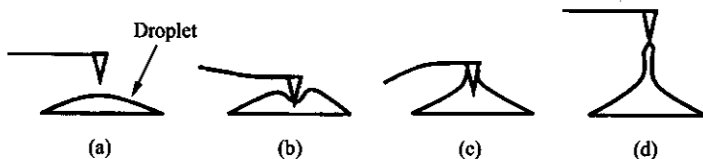
Fig. 2 Schematic illustration of AFM-tip indentation onto the melt droplet
